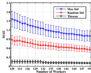
Figure 4: MAE comparison (setting III)
