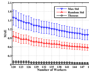
Figure 2: MAE comparison (setting I)
